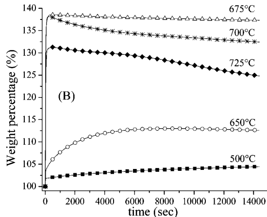
Figure 7. Isotherms of CO 2 sorption on 30-Li 2 CuO 2 , at different temperatures into a flux of CO 2 . (A) Isotherms obtained between 350 and 500 °C. (B) Isotherms obtained between 500 and 725 °C.
